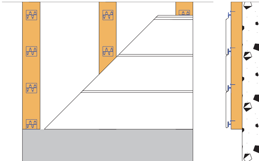
Installation with Thermory® clips
